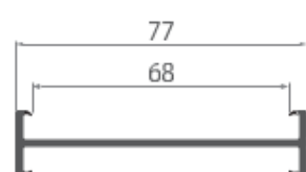
074 H-connector
