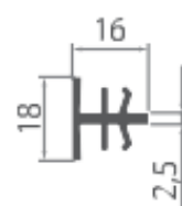
024 H-connector
