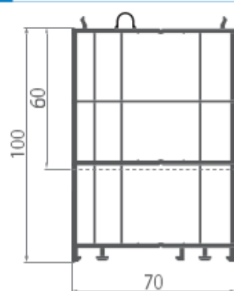
070 Frame extension
