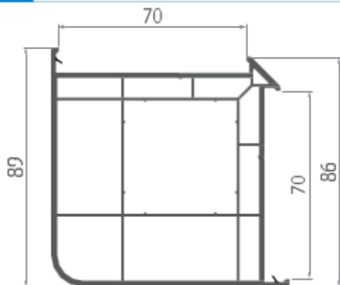
069 Corner adaptor
