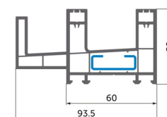
Sash adaptor SL Adaptor de hoja SL
