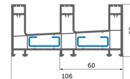
Frame SL 106/50 Marco SL 106/50 096
