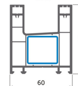
Frame SL 60/66 Marco SL 60/66 095
